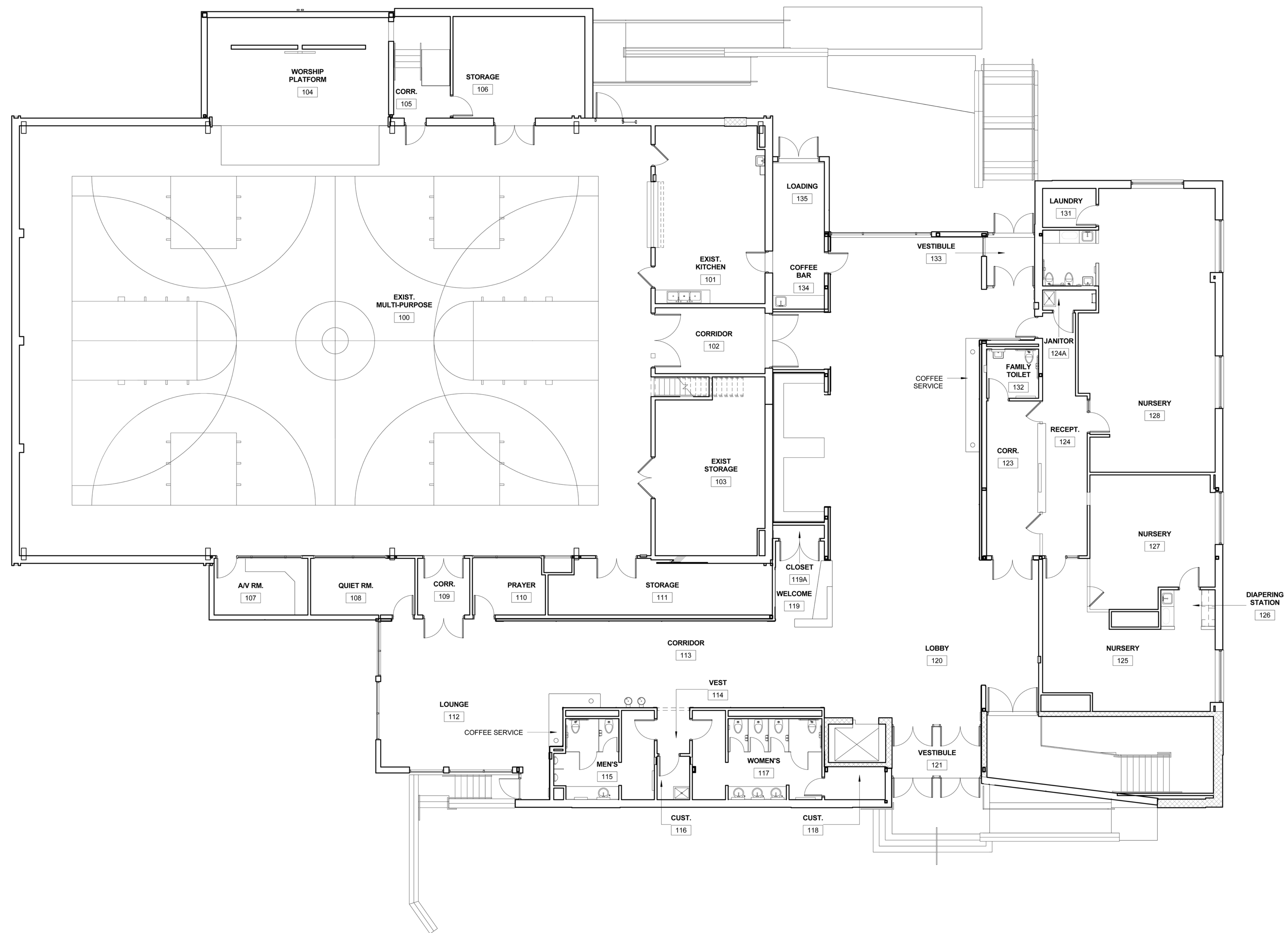
COLUMBIA PRESBYTERIAN CHURCH - MAIN LEVEL
